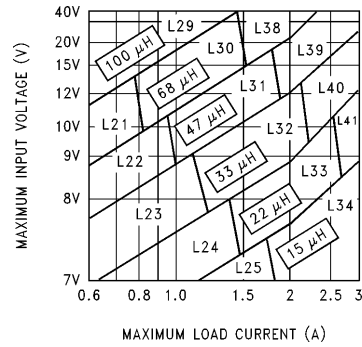
FIGURE 6. LM2596-5.0
