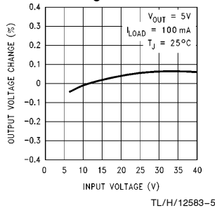
Line Regulation
