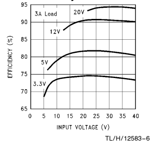
Efficiency
