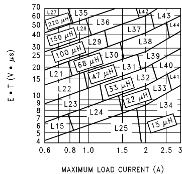
FIGURE 8. LM2596-ADJ
